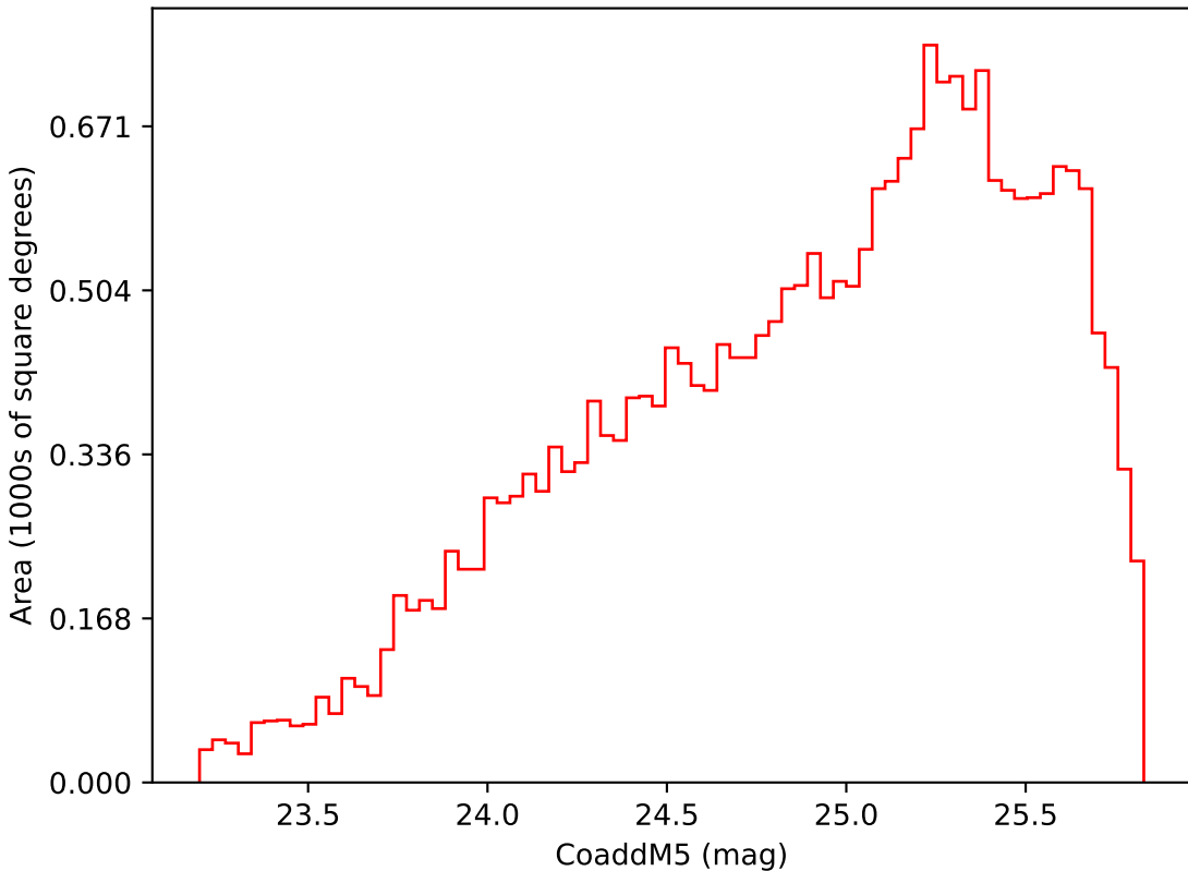
weather_cloudso4v3.4_10yrs Yr 3-4 i band: CoaddM5
