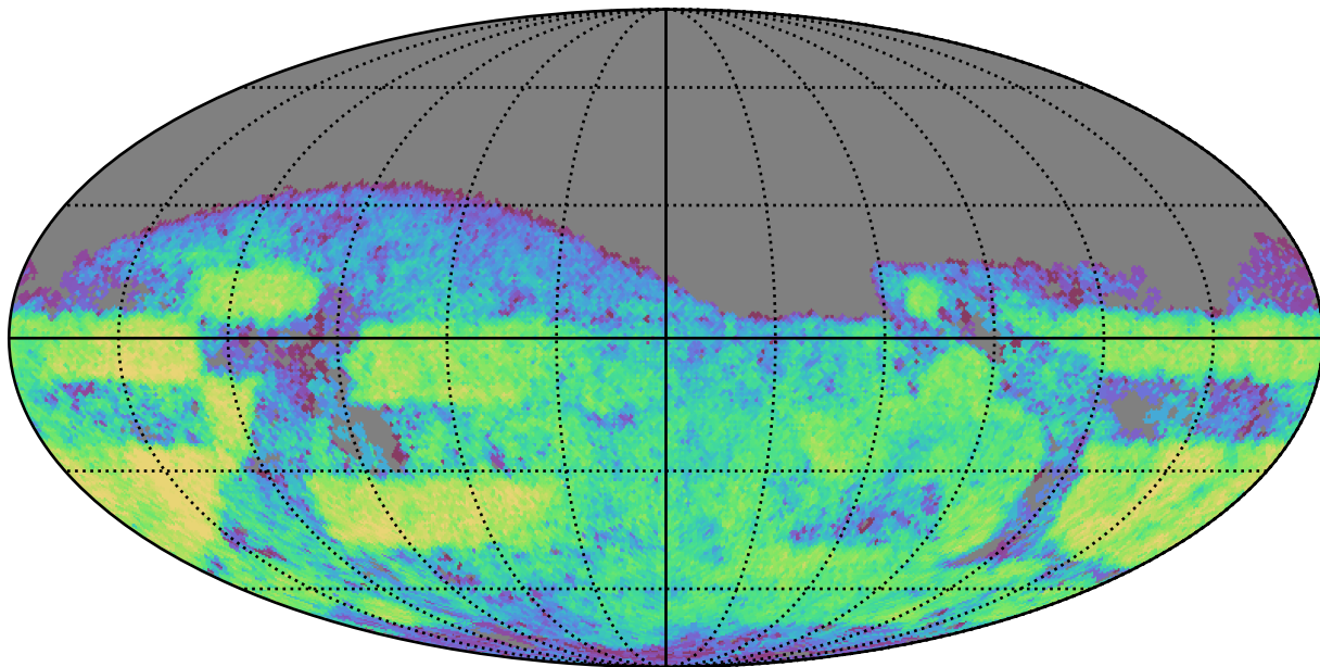
weather_cloudso4v3.4_10yrs Yr 3-4 g band: CoaddM5
