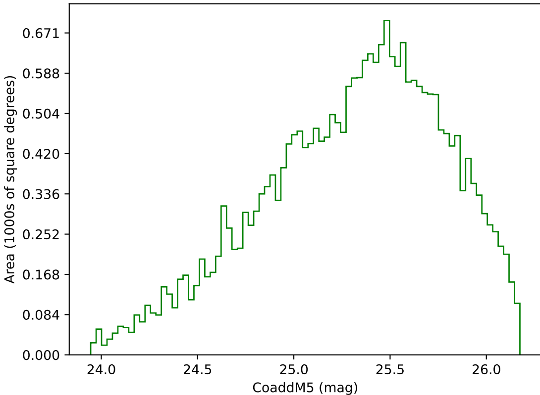
weather_cloudso4v3.4_10yrs Yr 3-4 g band: CoaddM5
