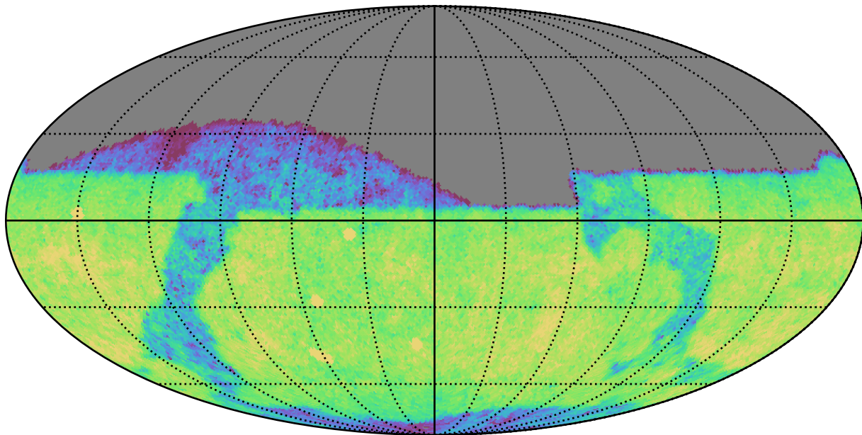
weather_cloudso4v3.4_10yrs Yr 1 z band: CoaddM5
