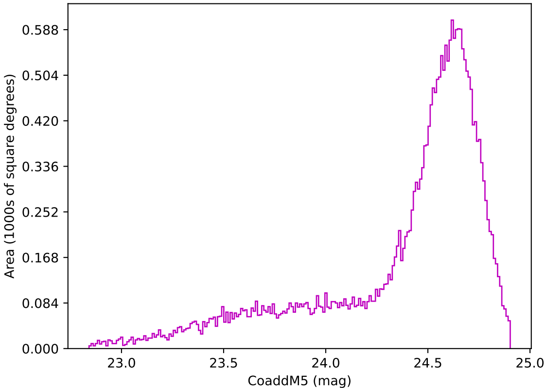
weather_cloudso4v3.4_10yrs Yr 1 z band: CoaddM5
