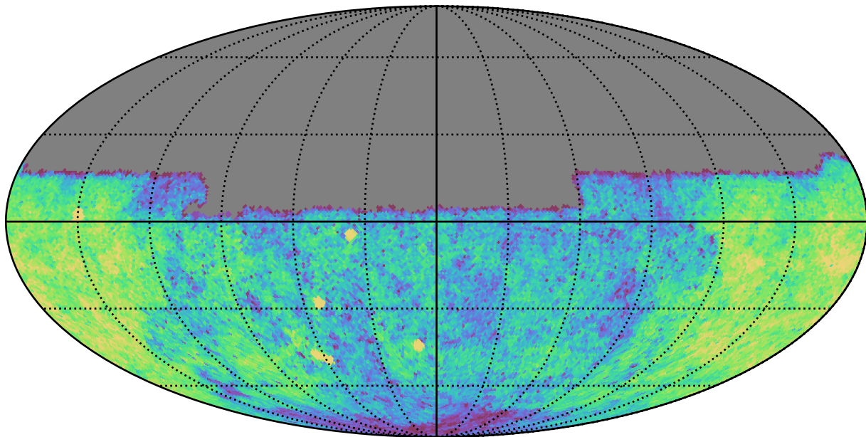
weather_cloudso4v3.4_10yrs Yr 1 u band: CoaddM5
