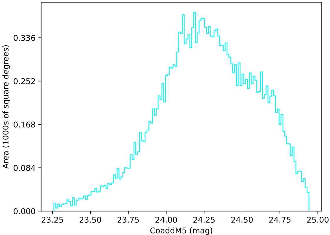
weather_cloudso4v3.4_10yrs Yr 1 u band: CoaddM5
