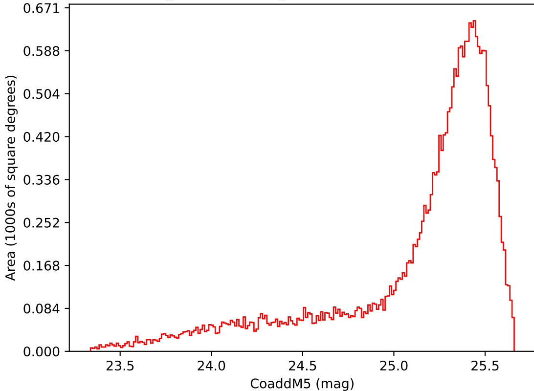
weather_cloudso4v3.4_10yrs Yr 1 i band: CoaddM5
