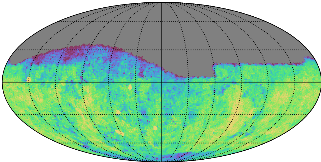
weather_cloudso4v3.4_10yrs Yr 1 g band: CoaddM5
