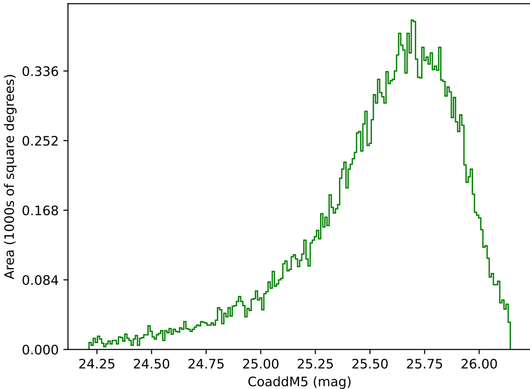
weather_cloudso4v3.4_10yrs Yr 1 g band: CoaddM5
