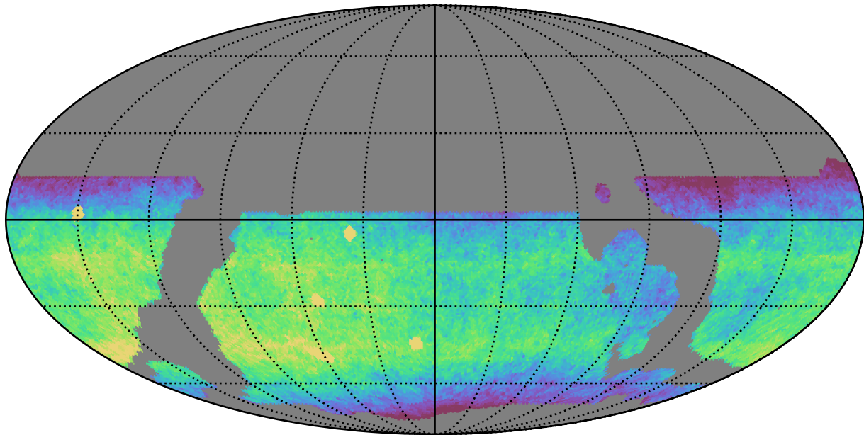
weather_cloudso4v3.4_10yrs WFD z band: CoaddM5
