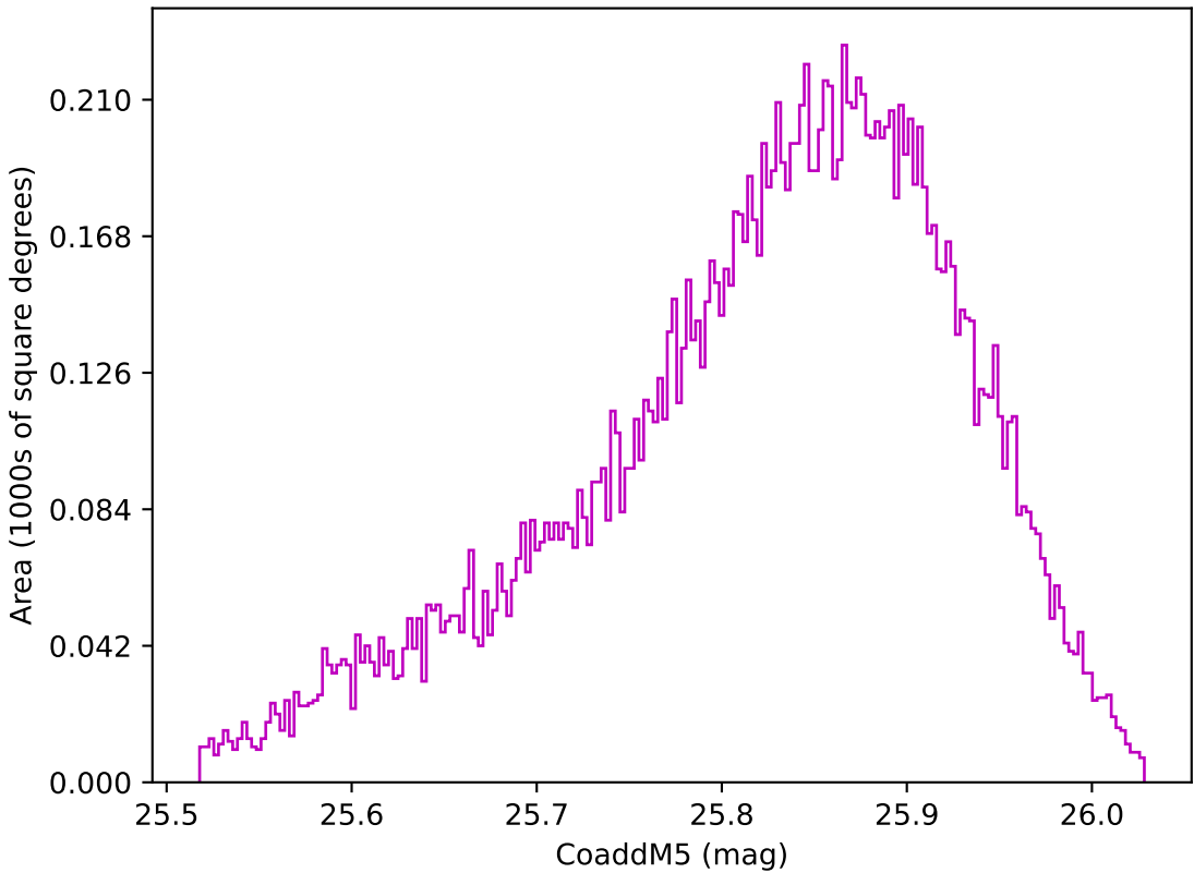
weather_cloudso4v3.4_10yrs WFD z band: CoaddM5
