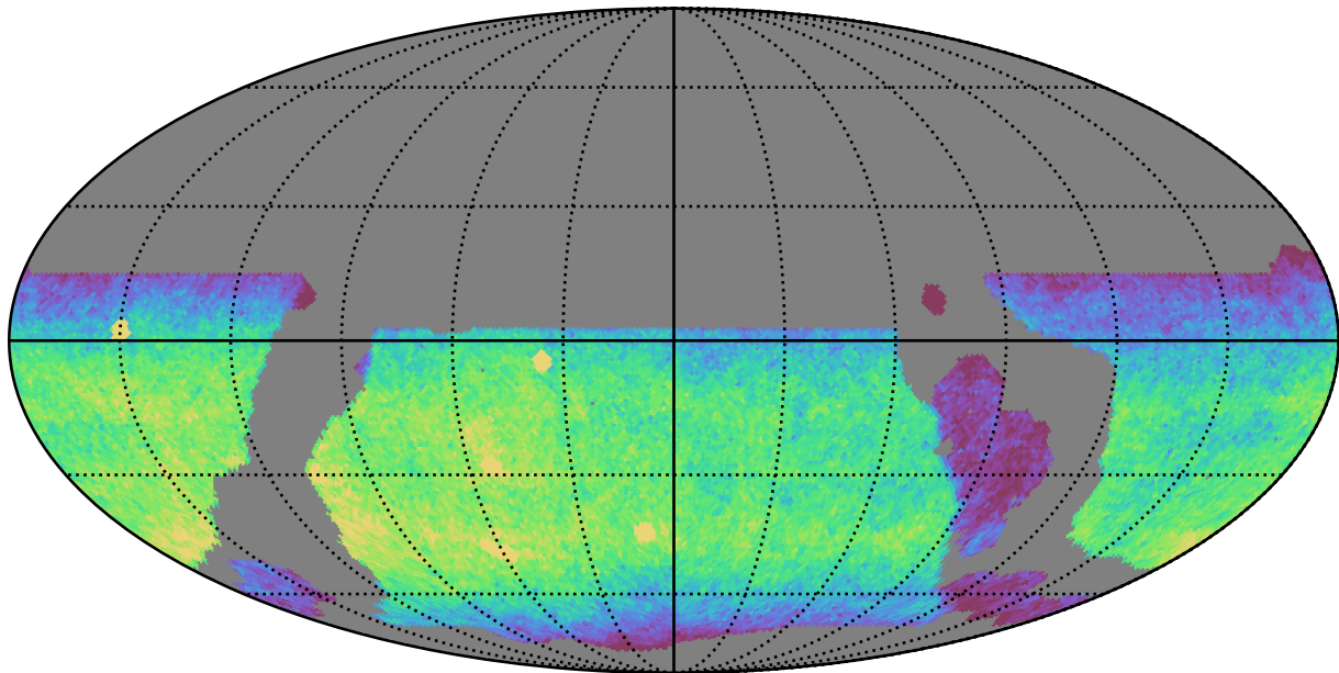
weather_cloudso4v3.4_10yrs WFD y band: CoaddM5
