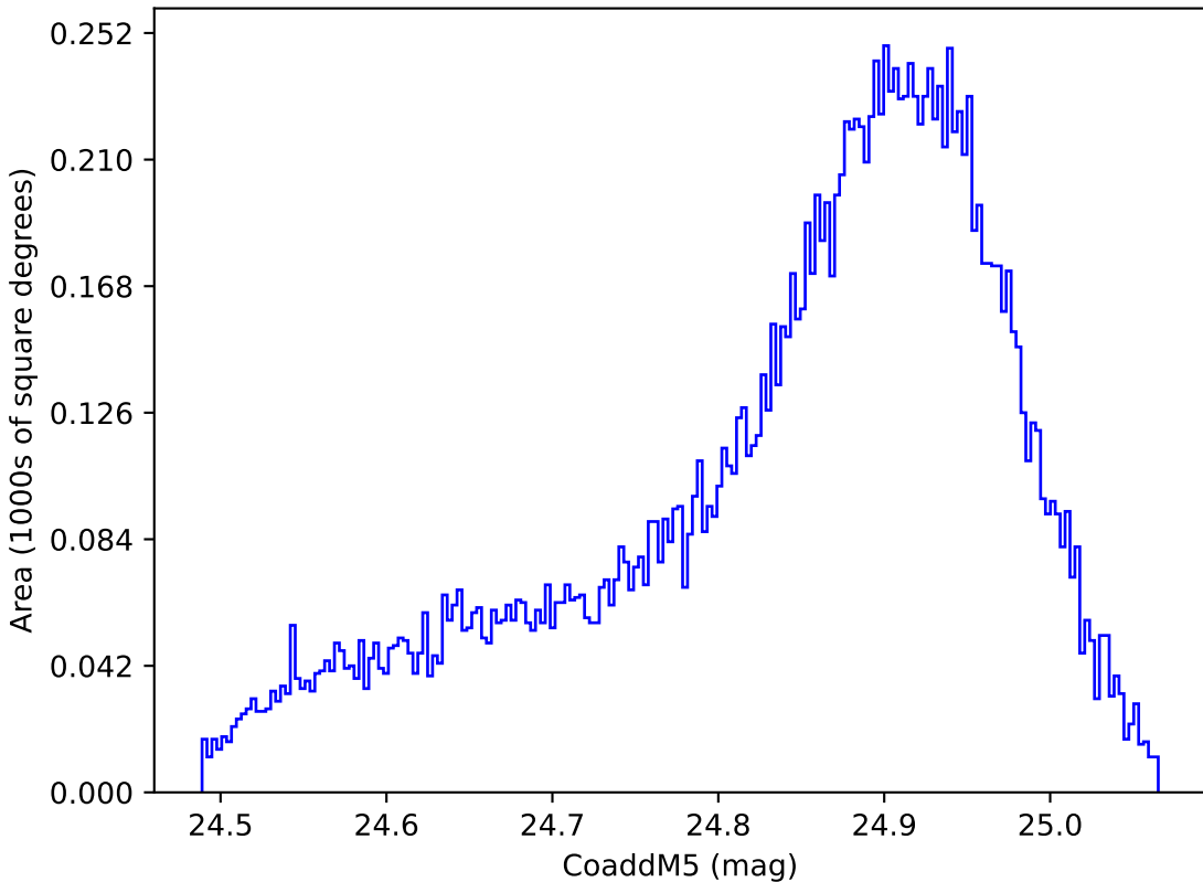
weather_cloudso4v3.4_10yrs WFD y band: CoaddM5
