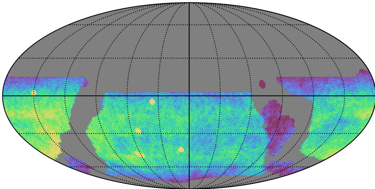
weather_cloudso4v3.4_10yrs WFD u band: CoaddM5
