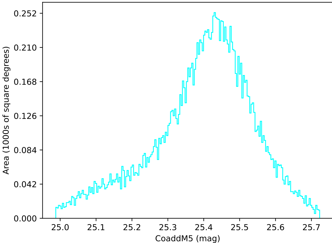
weather_cloudso4v3.4_10yrs WFD u band: CoaddM5
