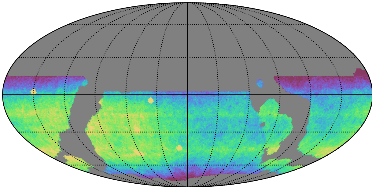
weather_cloudso4v3.4_10yrs WFD r band: CoaddM5
