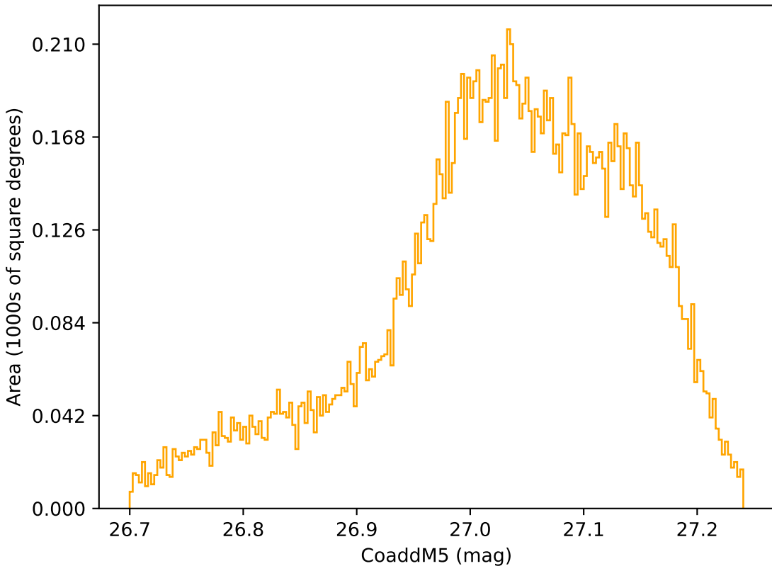
weather_cloudso4v3.4_10yrs WFD r band: CoaddM5
