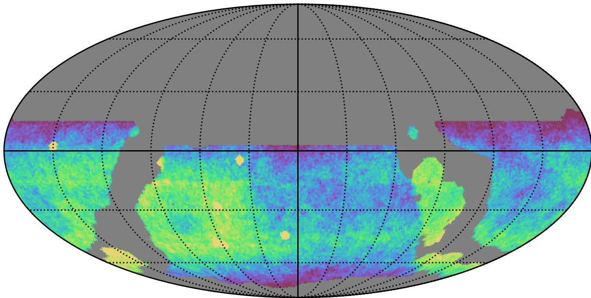
weather_cloudso4v3.4_10yrs WFD g band: CoaddM5
