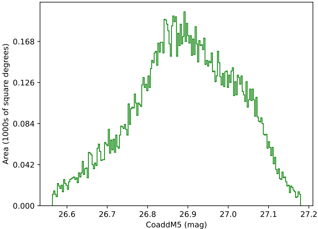
weather_cloudso4v3.4_10yrs WFD g band: CoaddM5
