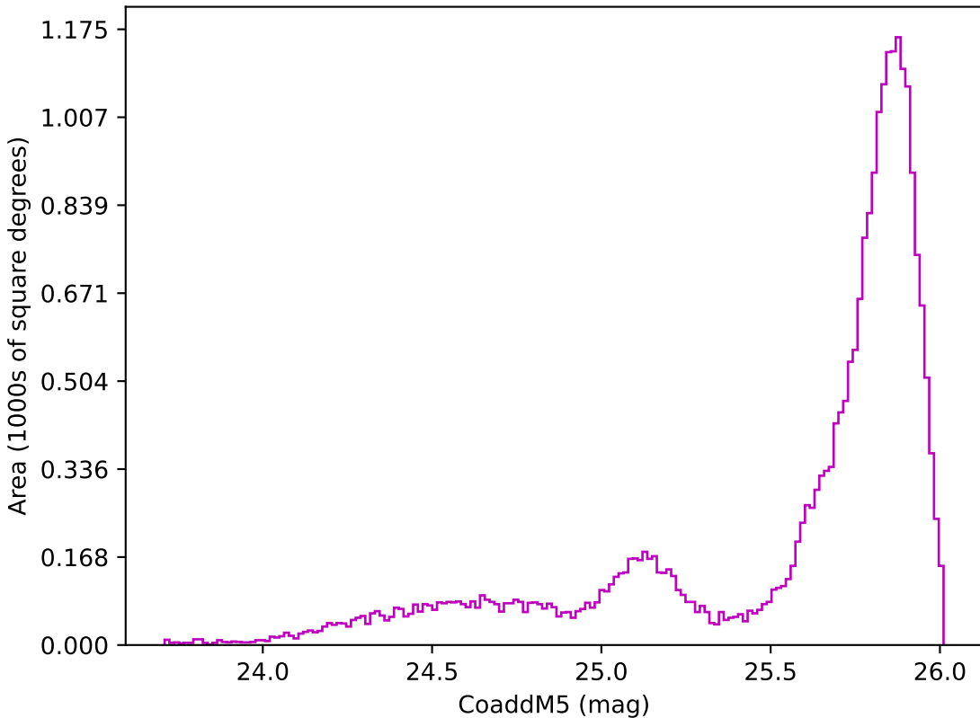
weather_cloudso4v3.4_10yrs All sky z band: CoaddM5
