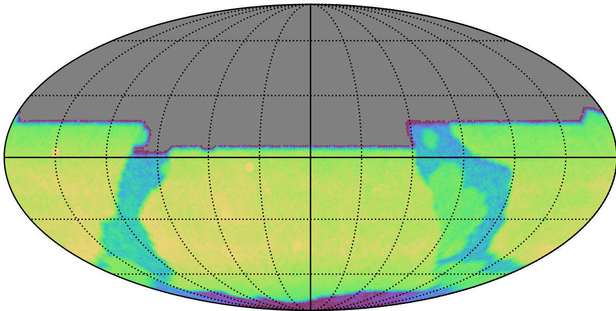
weather_cloudso4v3.4_10yrs All sky y band: CoaddM5
