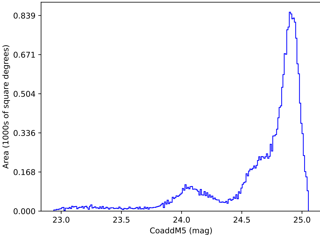
weather_cloudso4v3.4_10yrs All sky y band: CoaddM5
