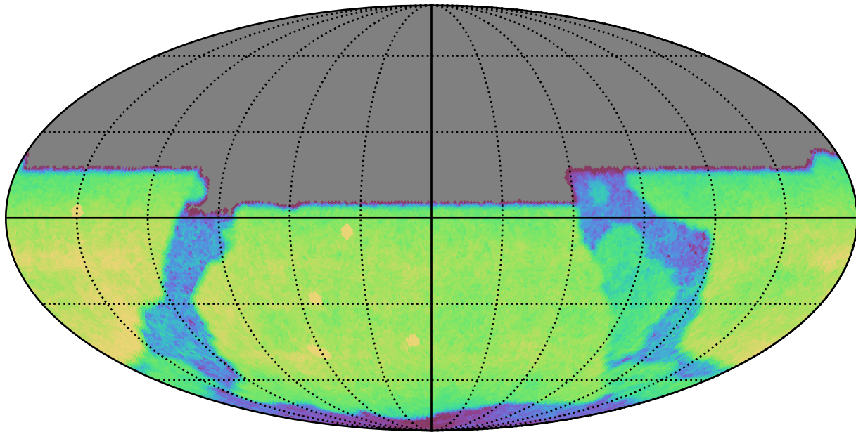
weather_cloudso4v3.4_10yrs All sky u band: CoaddM5
