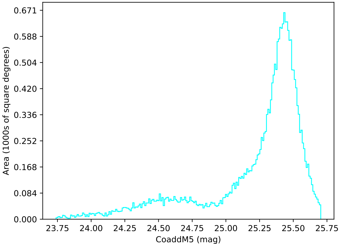
weather_cloudso4v3.4_10yrs All sky u band: CoaddM5
