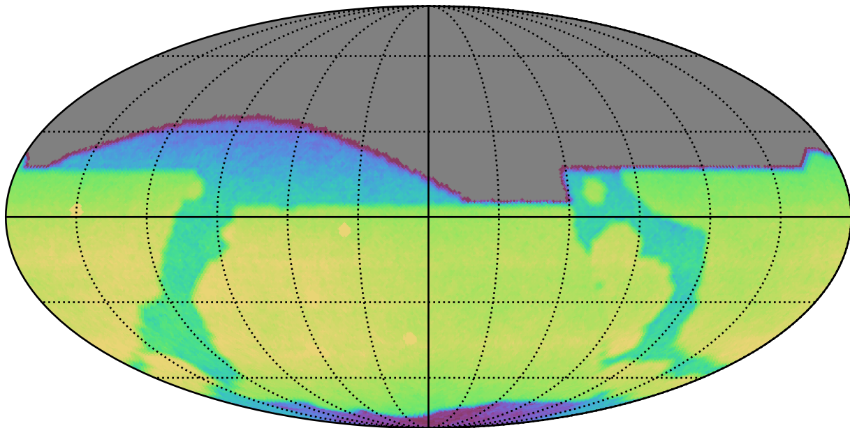
weather_cloudso4v3.4_10yrs All sky r band: CoaddM5
