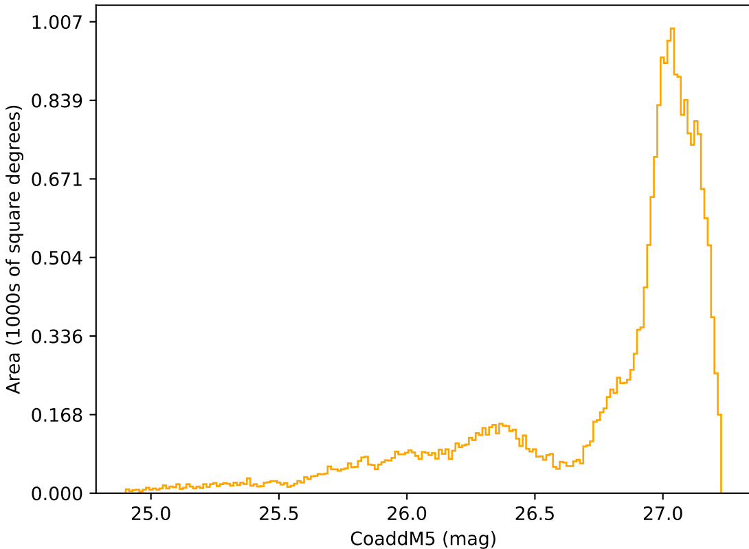
weather_cloudso4v3.4_10yrs All sky r band: CoaddM5
