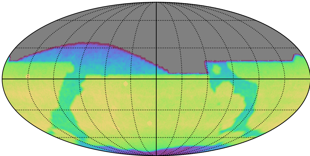
weather_cloudso4v3.4_10yrs All sky i band: CoaddM5
