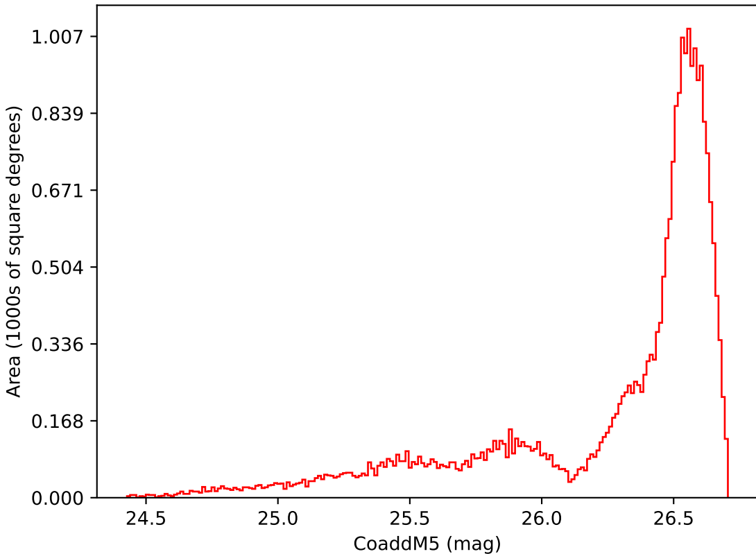
weather_cloudso4v3.4_10yrs All sky i band: CoaddM5
