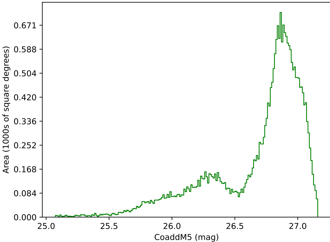
weather_cloudso4v3.4_10yrs All sky g band: CoaddM5
