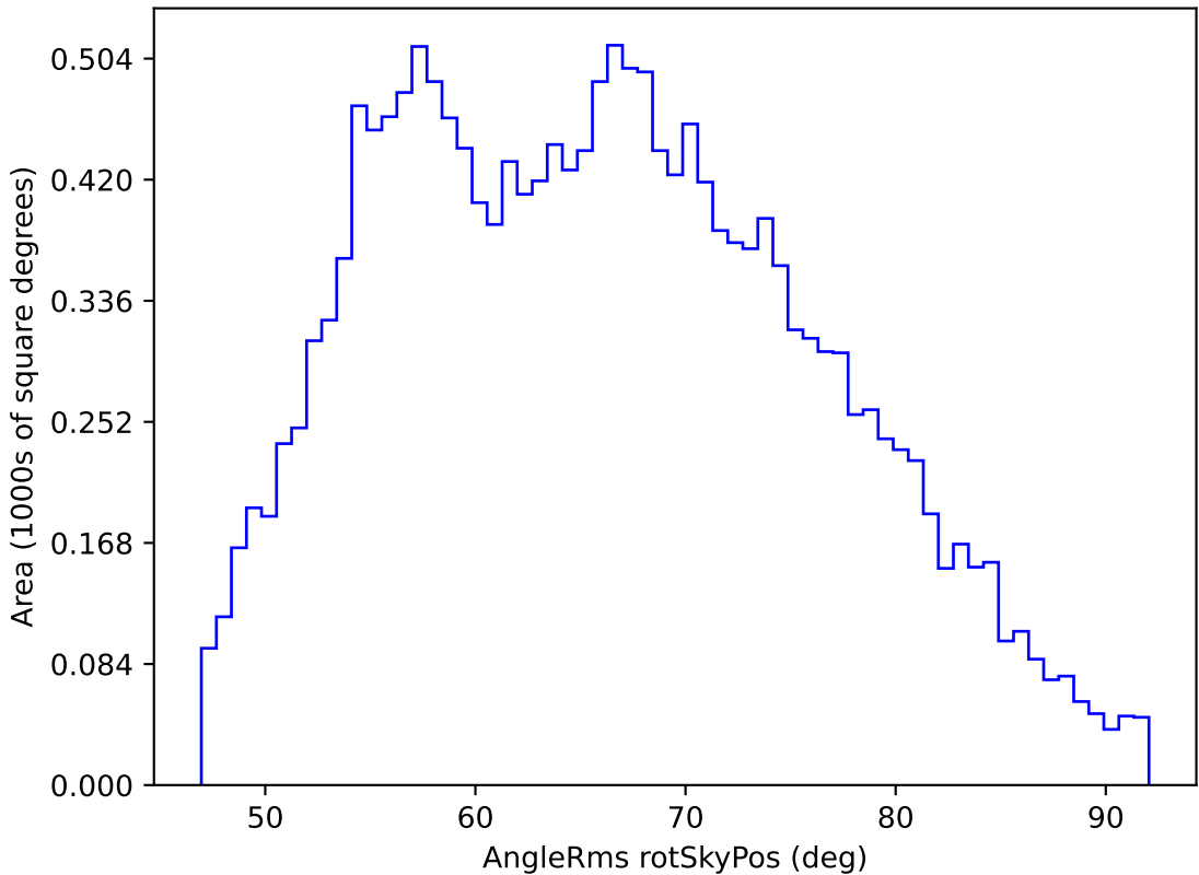
weather_cloudso4v3.4_10yrs WFD z band: AngleRms rotSkyPos
