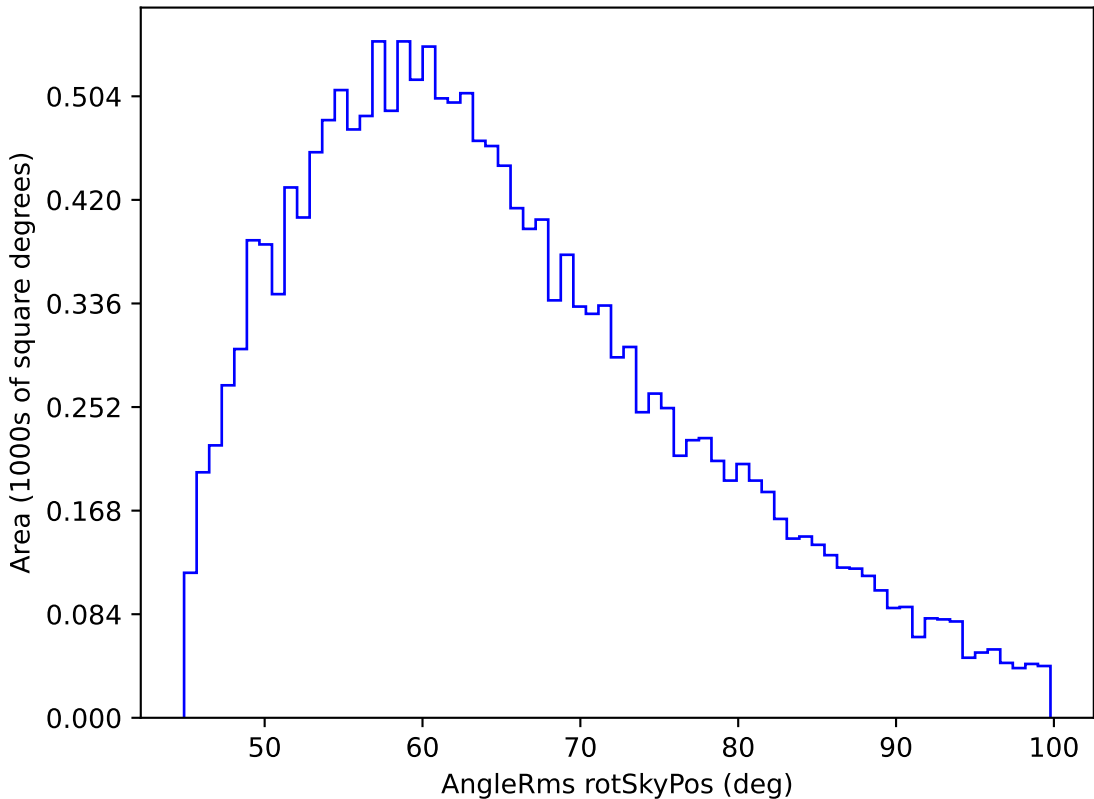
weather_cloudso4v3.4_10yrs WFD u band: AngleRms rotSkyPos
