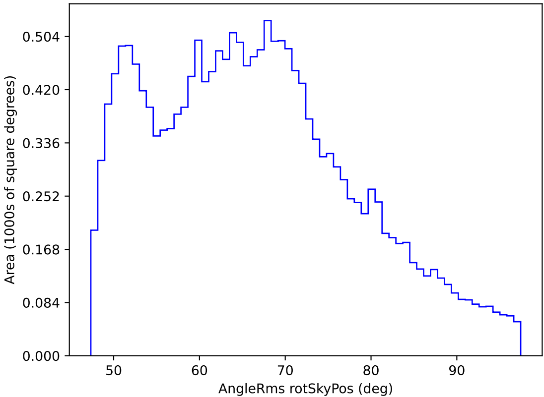
weather_cloudso4v3.4_10yrs WFD r band: AngleRms rotSkyPos
