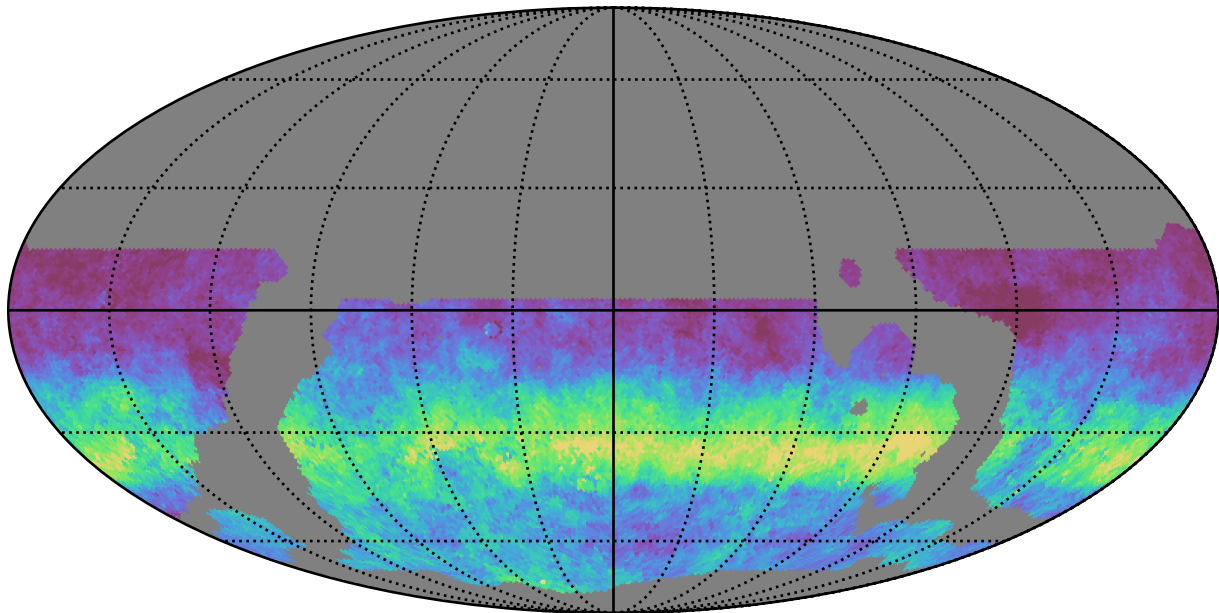
weather_cloudso4v3.4_10yrs WFD g band: AngleRms rotSkyPos
