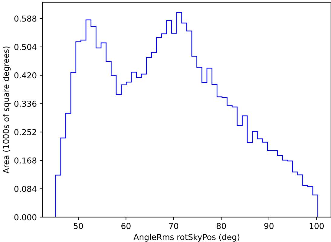
weather_cloudso4v3.4_10yrs WFD g band: AngleRms rotSkyPos
