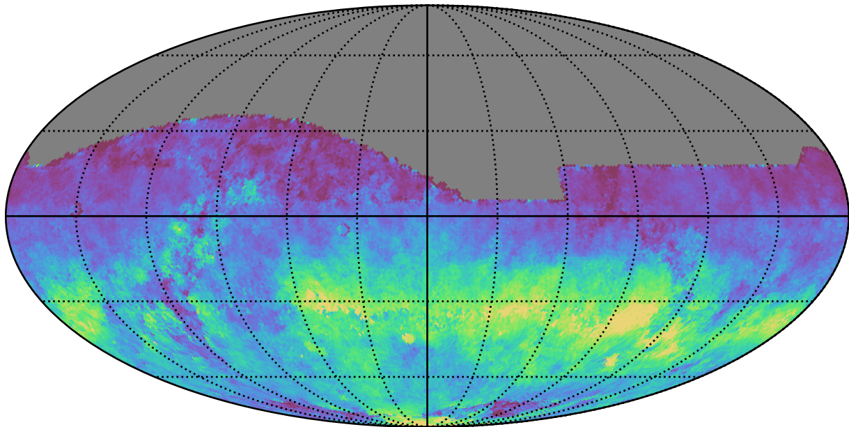
weather_cloudso4v3.4_10yrs All sky z band: AngleRms rotSkyPos
