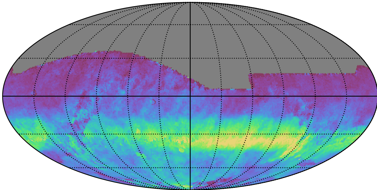
weather_cloudso4v3.4_10yrs All sky r band: AngleRms rotSkyPos
