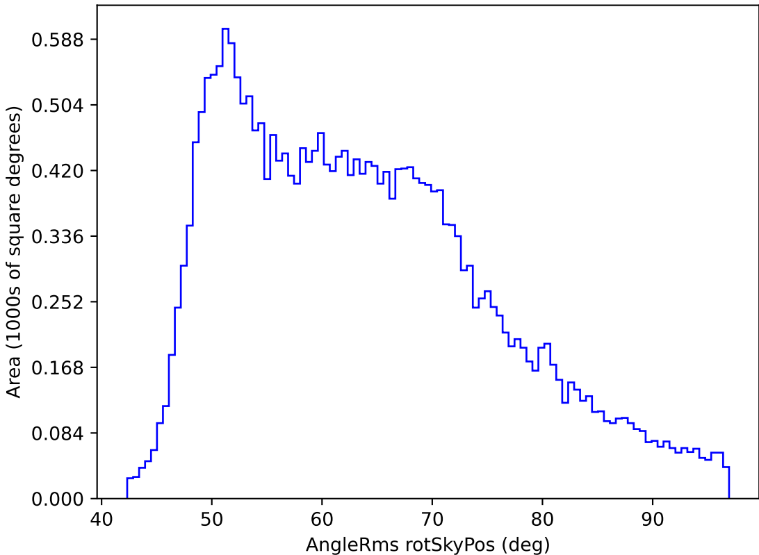
weather_cloudso4v3.4_10yrs All sky r band: AngleRms rotSkyPos
