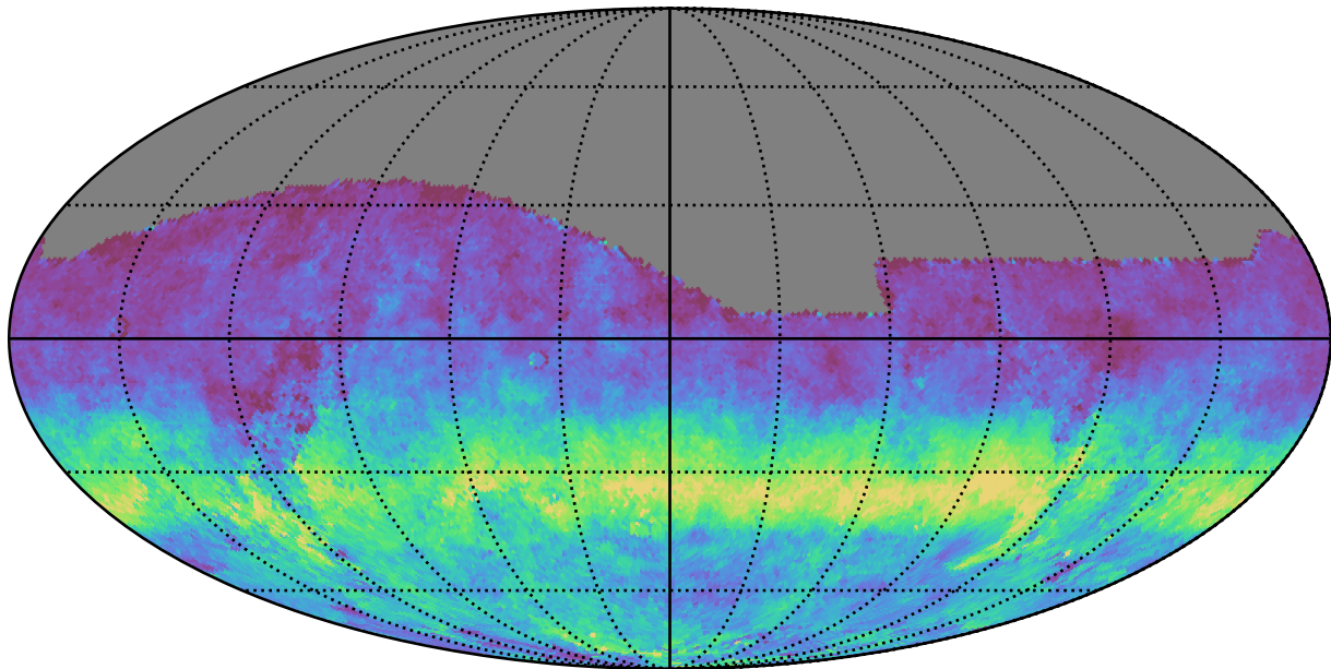
weather_cloudso4v3.4_10yrs All sky g band: AngleRms rotSkyPos
