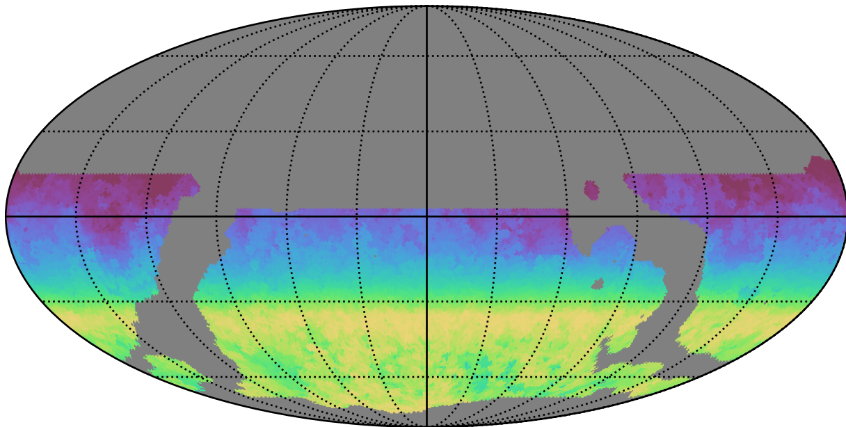
weather_cloudso4v3.4_10yrs WFD all bands: AngleRange rotSkyPos
