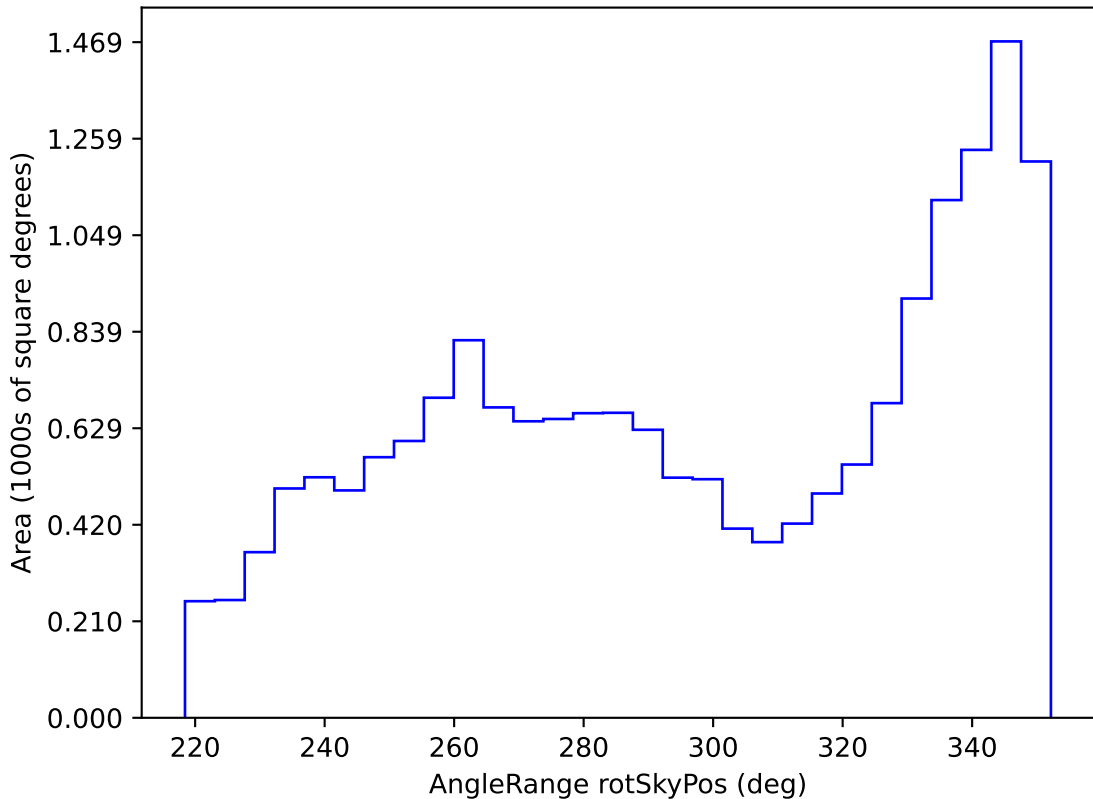
weather_cloudso4v3.4_10yrs WFD all bands: AngleRange rotSkyPos
