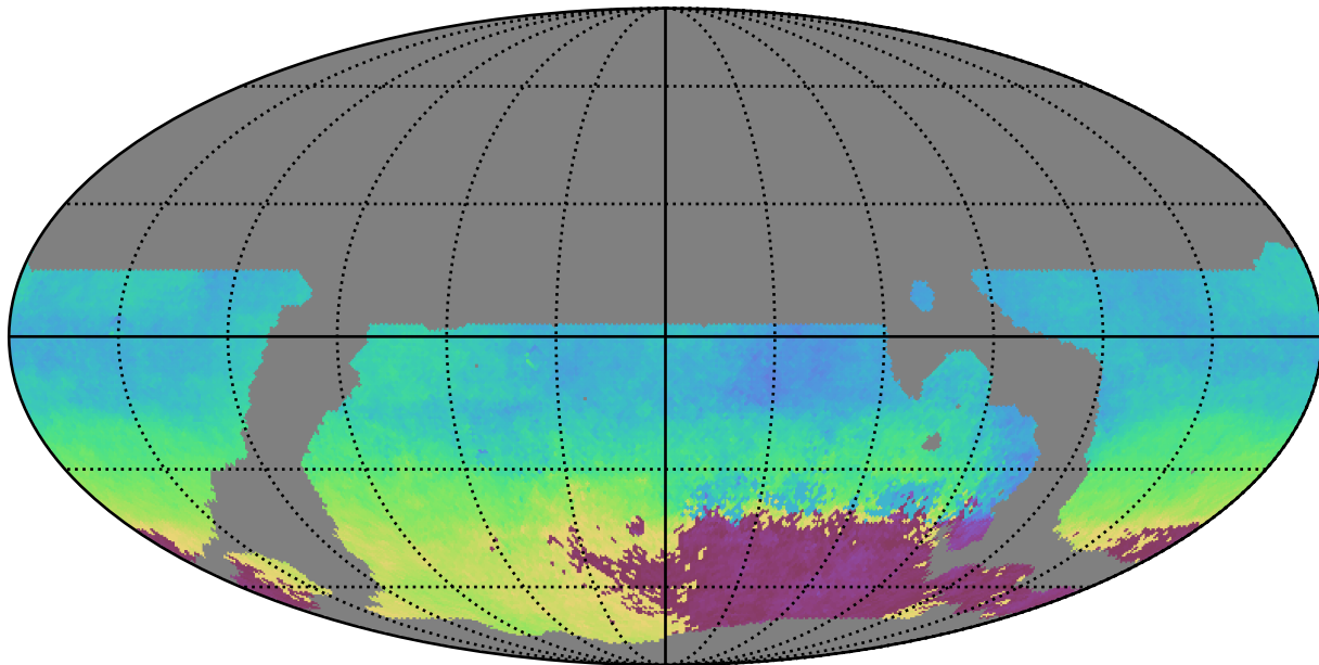
weather_cloudso4v3.4_10yrs WFD u band: AngleMean rotSkyPos
