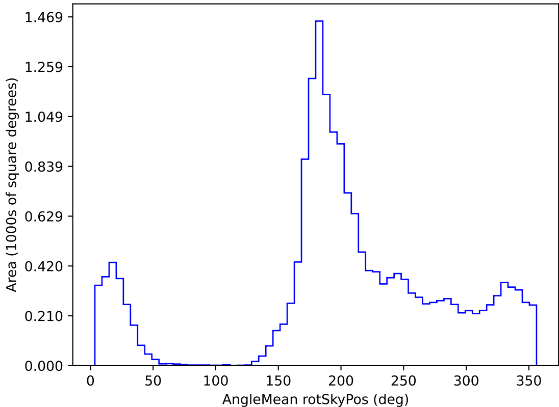
weather_cloudso4v3.4_10yrs WFD u band: AngleMean rotSkyPos
