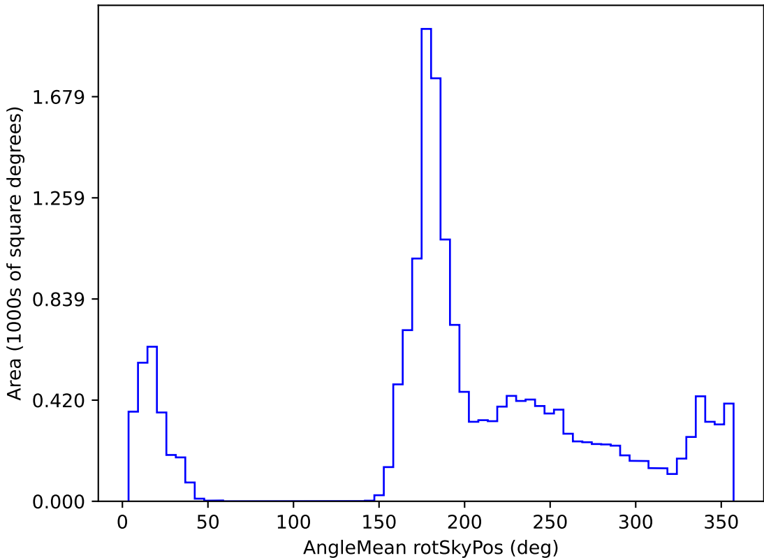
weather_cloudso4v3.4_10yrs WFD r band: AngleMean rotSkyPos
