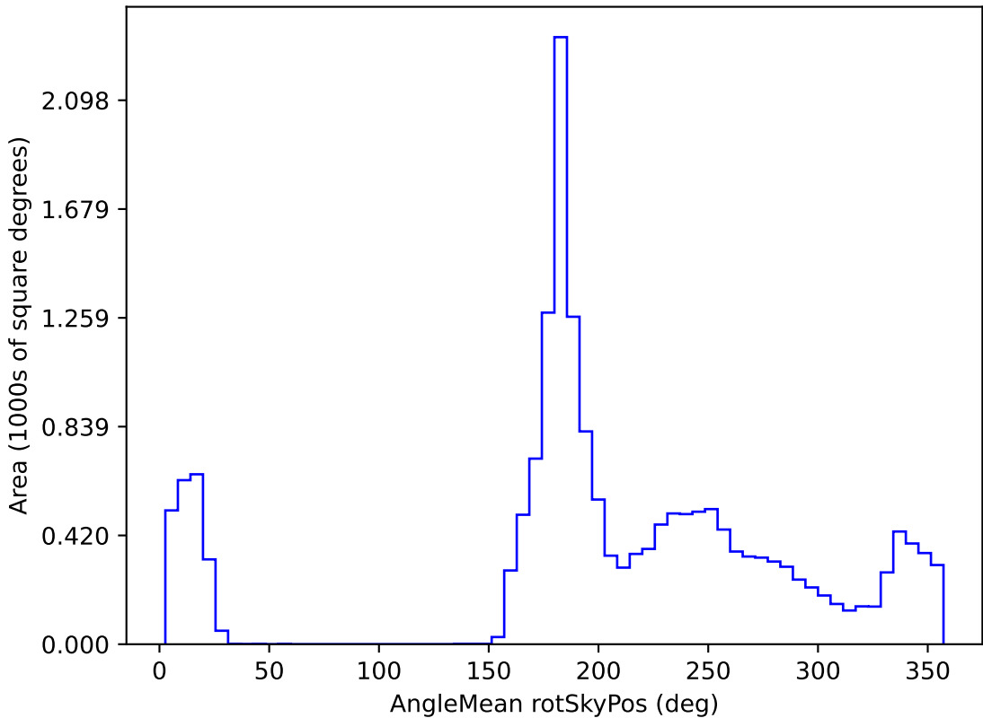
weather_cloudso4v3.4_10yrs WFD all bands: AngleMean rotSkyPos
