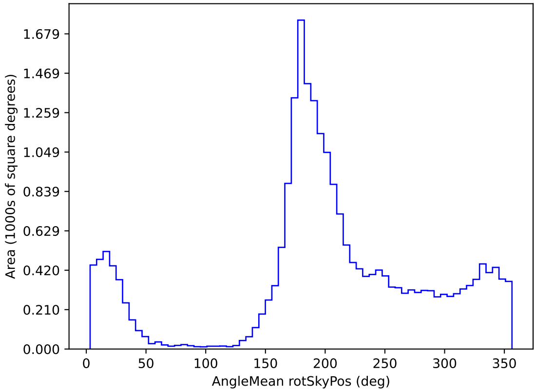
weather_cloudso4v3.4_10yrs All sky u band: AngleMean rotSkyPos
