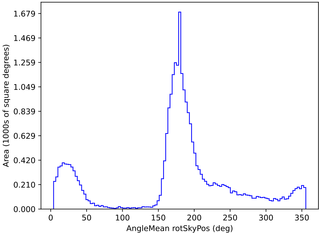
weather_cloudso4v3.4_10yrs All sky g band: AngleMean rotSkyPos
