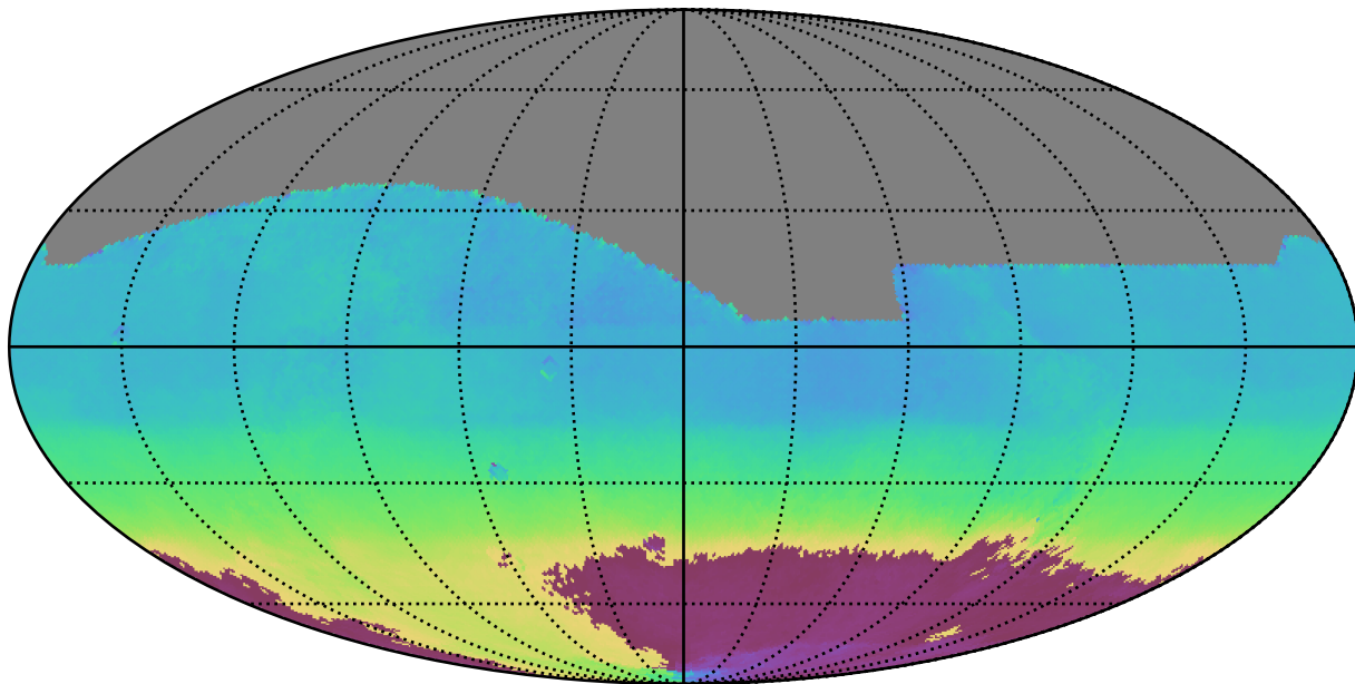
weather_cloudso4v3.4_10yrs All sky all bands: AngleMean rotSkyPos
