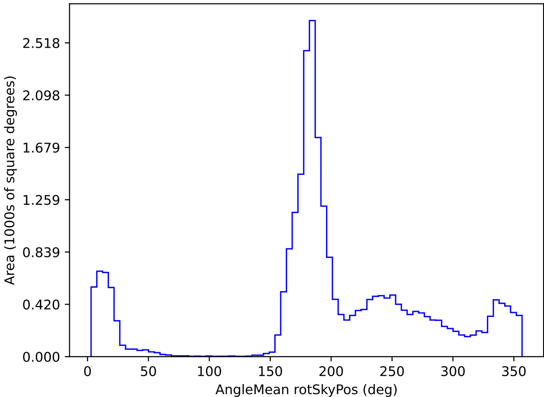
weather_cloudso4v3.4_10yrs All sky all bands: AngleMean rotSkyPos
