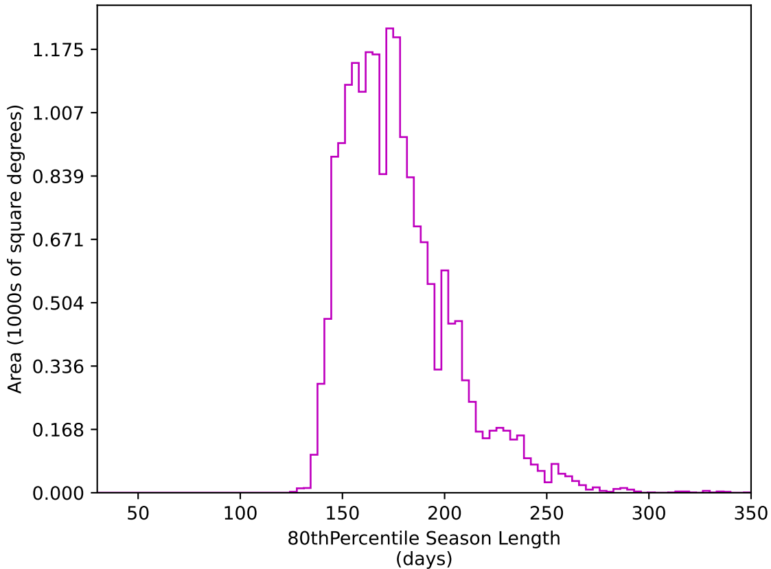
weather_cloudso4v3.4_10yrs WFD z band: 80thPercentile Season Length
